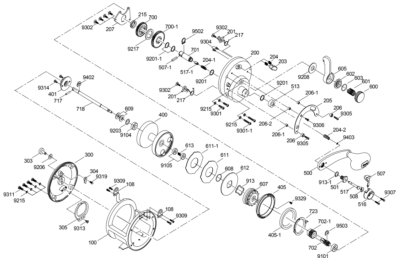
TG - 15 - II (1 of 2) Spare Parts
